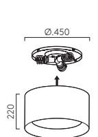
BEVEL ROUND 450
