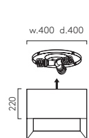
BEVEL SQUARE 400
