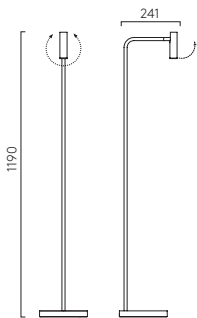
ENNA FLOOR
